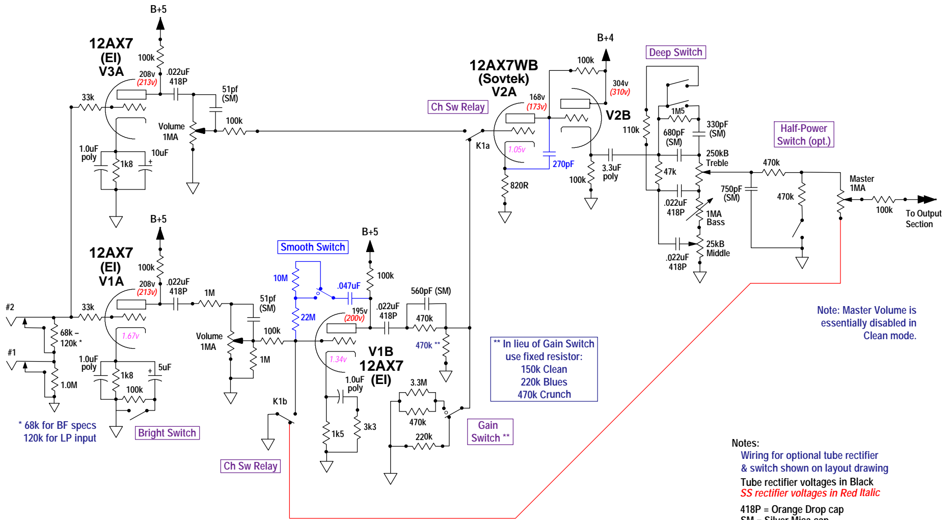
Channel Switching variation B (Preamp section)
